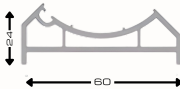
Bay Pole Adapter AST67- WH
