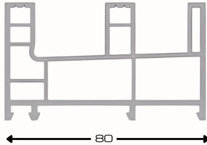
Sliding 2.5 Track Frame AST43- WH
