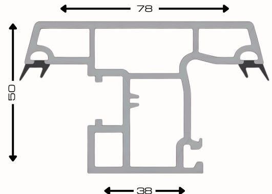
Casement Window Sash - Grill AST04-WHG
