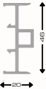
Connector - 66/80 Sash AST27- WH
