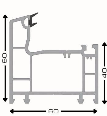
Casement Frame AST01-WHG
