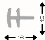
Frame Connector AST54- WH
