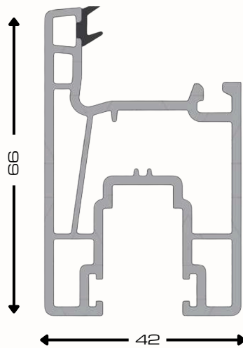
Sliding Sash 66mm AST16- WHG
