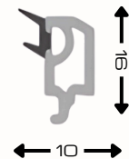
Glazing Bead 10mm AST37- WHG
