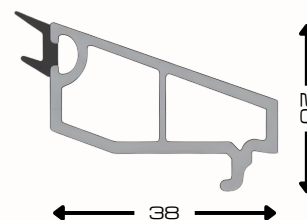
Glazing Bead 35mm AST31-WHG
