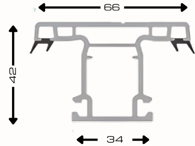
Sliding T Mullion - 66/80mm Sash AST21- WHG
