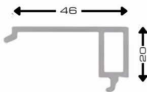
Louver Bead AST60- WH
