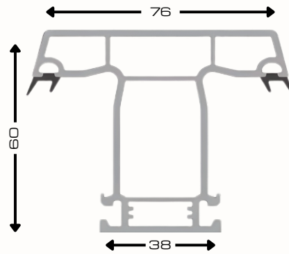
Casement T Mullion AST03-WHG
