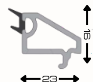
Glazing Bead 23mm AST36- WHG
