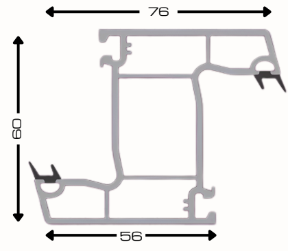
Casement Z Mullion AST07-WHG
