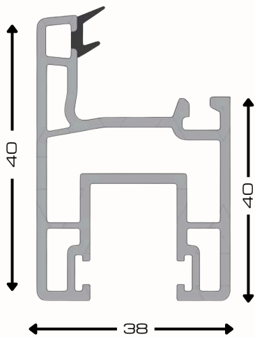
Sliding Sash 56mm AST15- WHG
