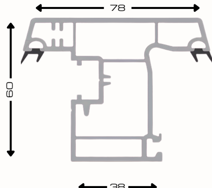
Casement Window Sash AST05-WHG
