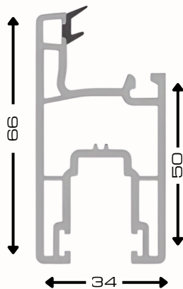
Sliding Sash for 80mm AST45- WHG
