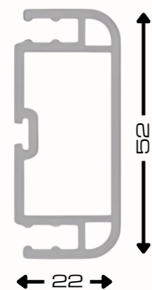
Bug Screen 52mm T Mullion AST24- WH
