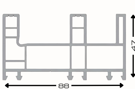
Sliding 2.5 Track Frame AST13- WH
