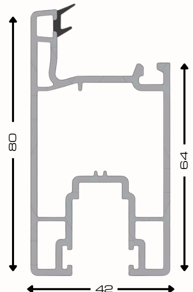
Sliding Sash 80mm AST17- WHG
