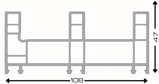
Sliding 3 Track Frame AST12- WH
