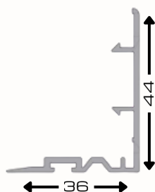
Interlock - 66/80 Sash AST19- WH
