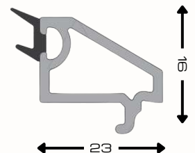
Glazing Bead 23mm AST36-WHG
