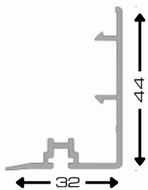
Interlock - 56 Sash AST18- WH
