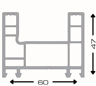
Sliding 2 Track Frame AST11- WH
