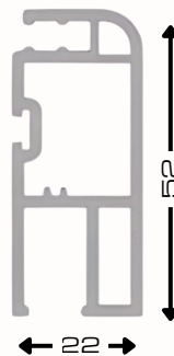
Bug Screen 52mm AST25- WH
