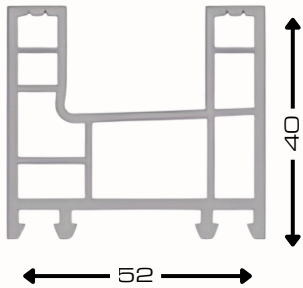
Sliding 2 Track Frame AST41- WH
